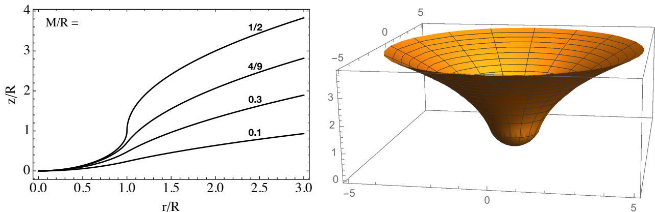
FIG. 1. Embedding of equatorial planes at fixed time into \mathbb{R}^3 . The 3-D plot is for M/R = 4/9 .
